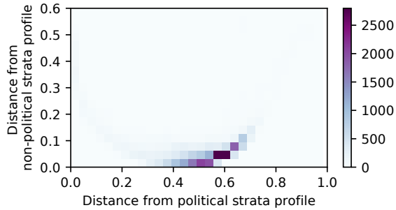
Figure 5: Density of subreddits by JSD(D_{\text{subr}}||D_{\text{pol}}) and JSD(D_{\text{subr}}||D_{\text{nonpol}}) scores. Few subreddits are equidistant from both strata profiles; most are close to the non-political strata profile.
